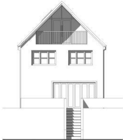
Rear Elevation 1 : 100
