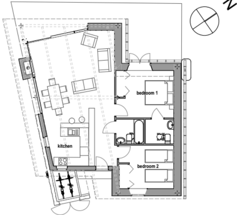
LODGE 1 & 2 PLANS
